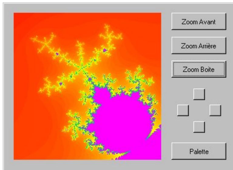
Applet Mendelscope
